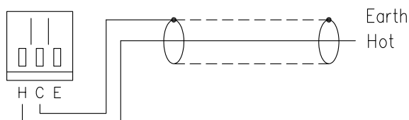
Connection Diagram
